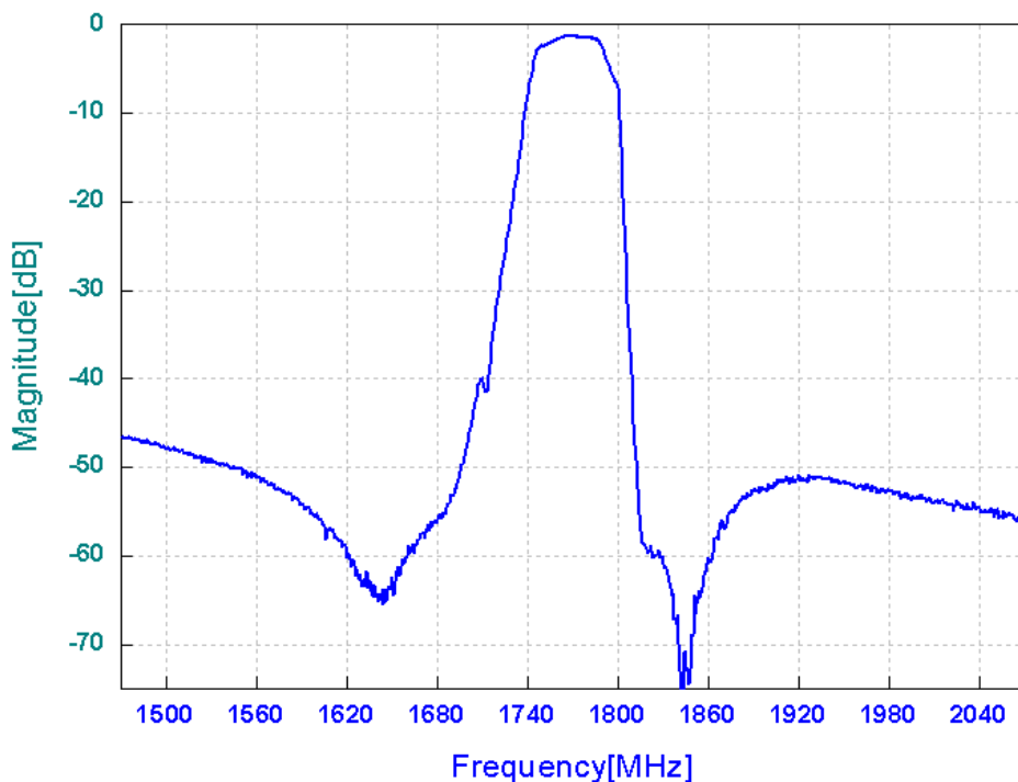
Frequency Response
